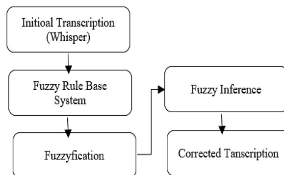
Fig. 1. Fuzzy rule-based architecture for ASR correction.
