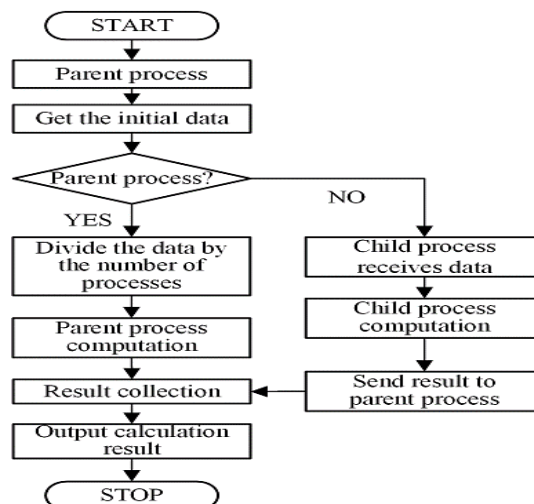
Fig. 5. Parallel computing algorithm flowchart [24].
